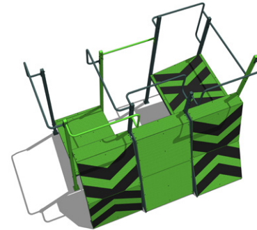
PS 03 PARKOUR SET JUMPER 3 711 x 2 923 x 3 000 mm
